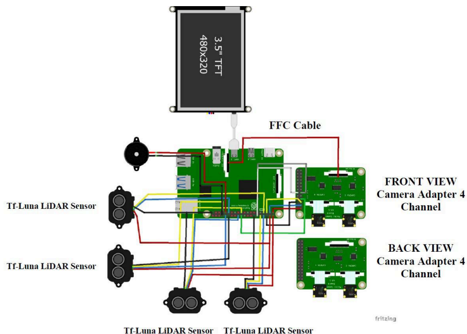
Figure 2. Schematic of Design IoT Board
