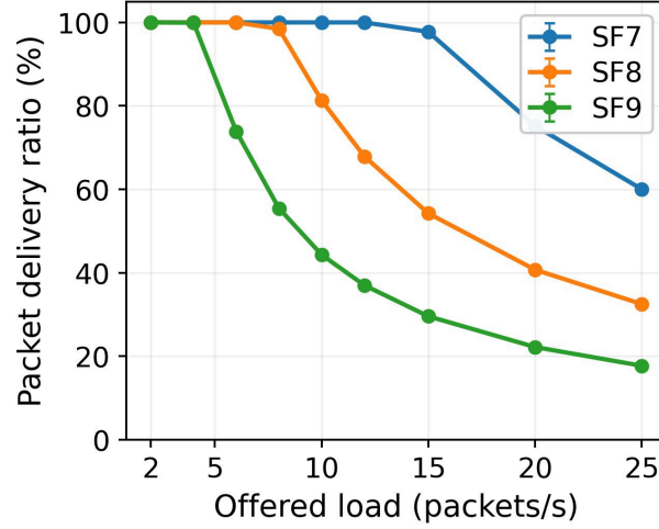
Figure 4. packet delivery ratio under varying load ( L_2 = 20 )
