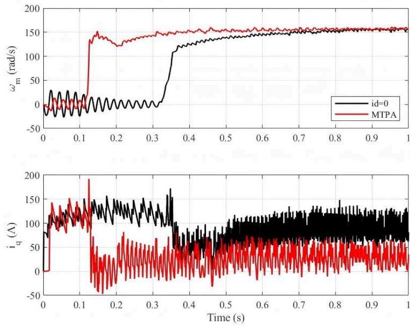
Figure 3. Speed and q-axis current during the 5→10 N·m load step at t = 0.5 s (black: id=0 control; red: MTPA).
