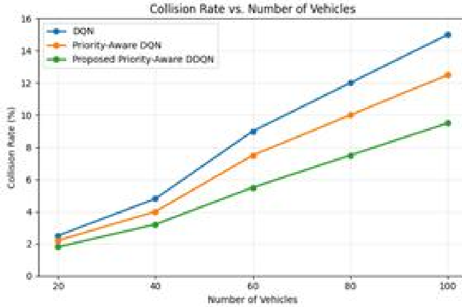
Figure 6. Resource collision rate versus the number of vehicles.
