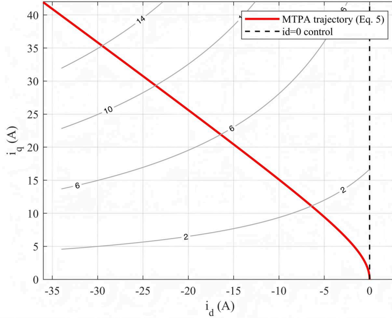
Figure 1. MTPA trajectory and constant-torque loci in the i_d - i_q plane (Table 1 parameters).
