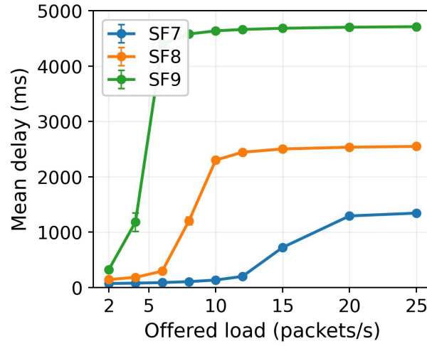
Figure 5. mean end-to-end delay under varying load ( L_2 = 20 )
