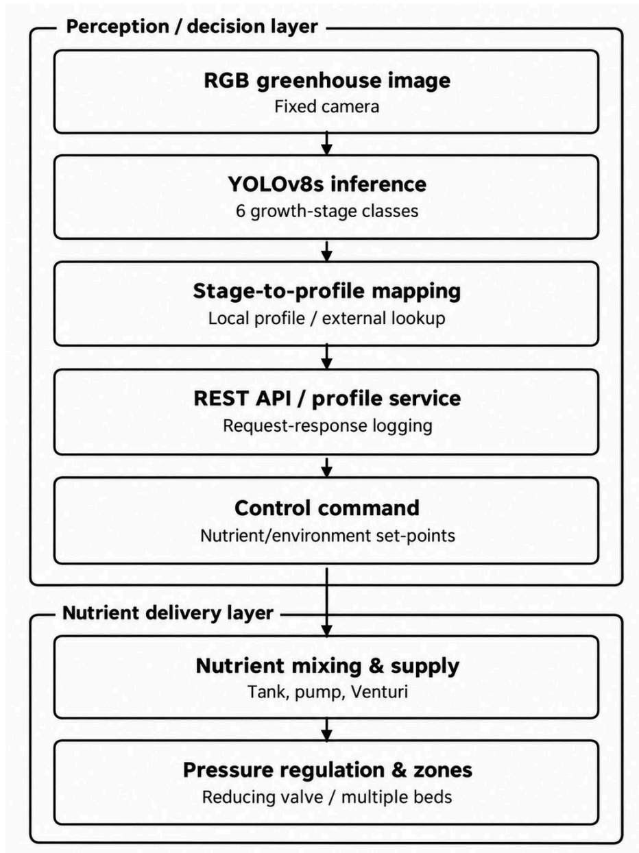
Figure 1. . Integrated perception-to-control architecture. The perception/decision layer follows the growth-stage concept of [10], while the nutrient-delivery layer is consistent with the actuation concept of [9].
