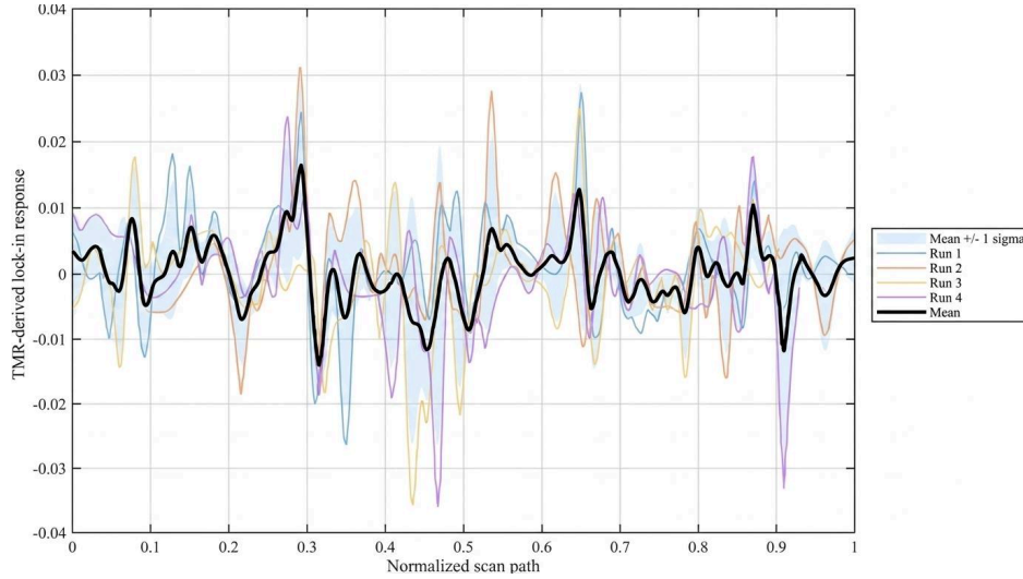
Figure 3. Signed phase-referenced TMR response for four repeated scans of the same ACF-bonded FFC specimen. The vertical axis is reported in arbitrary units because the complete calibration chain was not retained. The black trace and shaded band denote the mean and \pm 1\sigma , respectively.
