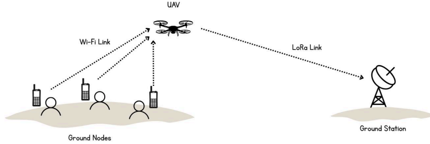
Figure 1. UAV-assisted hybrid Wi-Fi–LoRa emergency communication architecture: ground nodes ingest telemetry into the UAV over Wi-Fi; the UAV aggregates and relays packets across long ranges to a terrestrial LoRa gateway.
