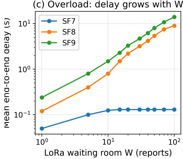
Figure 8. Mean end-to-end delay under varying LoRa buffer capacities for SF7, SF8, and SF9.
