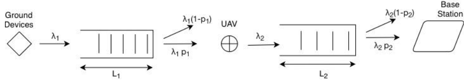
Figure 2. Two-stage tandem M/D/1 queueing model for the proposed Wi-Fi-LoRa relay. \lambda_1 and \lambda_2 denote the Wi-Fi and LoRa packet arrival rates; L_1 and L_2 represent their respective waiting-buffer capacities; TW and TL are the deterministic packet service times; \mu_1 = 1/TW and \mu_2 = 1/TL are the corresponding service rates. The probabilities of successful forwarding are p_1 and p_2 , with packet discard probabilities 1-p_1 and 1-p_2 . The departure rates are d_1 = \lambda_1 p_1 and d_2 = \lambda_2 p_2 , where \lambda_2 = d_1 .
