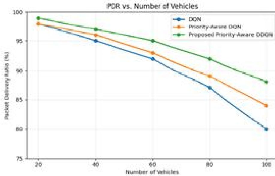
Figure 4. Packet delivery ratio versus the number of vehicles.
