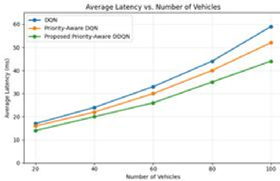
Figure 5. Average delivery latency versus the number of vehicles.
