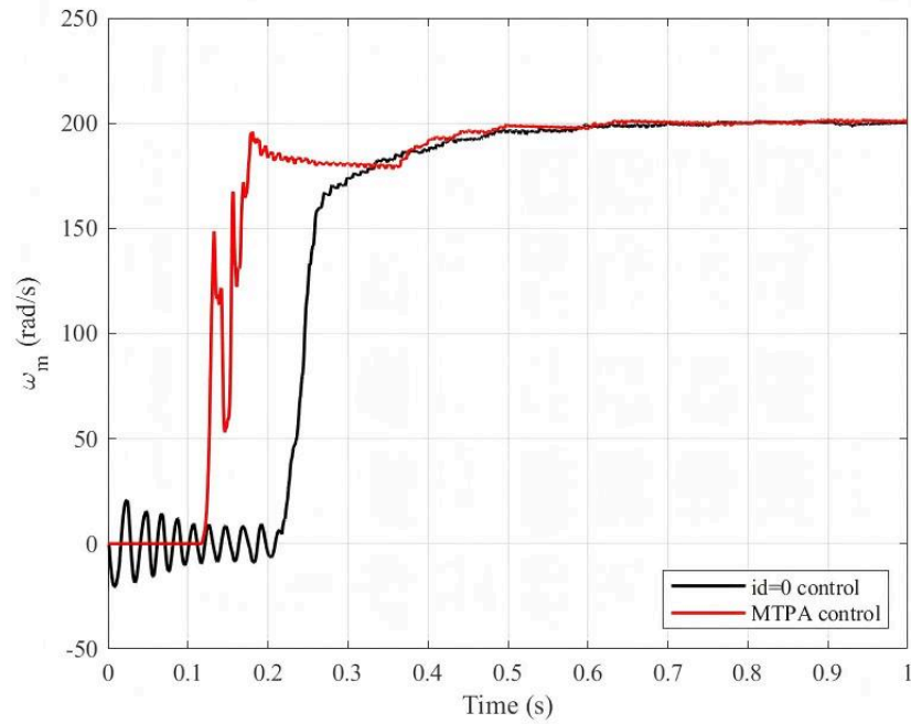
Figure 2. Speed responses to a no-load step to 200 rad/s (black: id=0 control; red: MTPA control).
