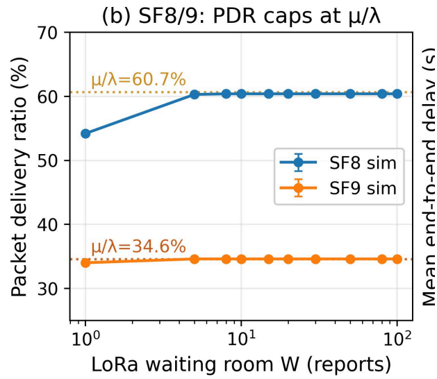
Figure 7. Packet delivery ratio and service-capacity limits for SF8 and SF9 under varying LoRa buffer capacities.
