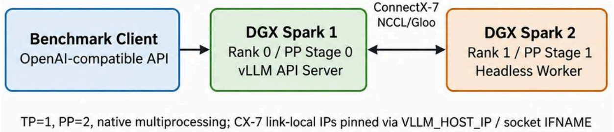
Figure 1. Final single-replica dual-node architecture used in the experiments.
