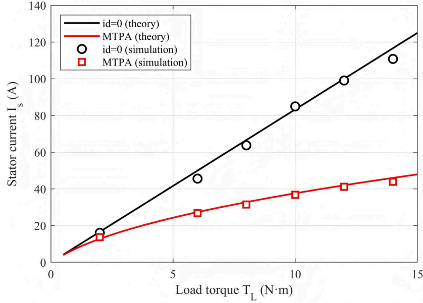
Figure 4. Stator-current magnitude versus load torque (theoretical curves with simulated points).
