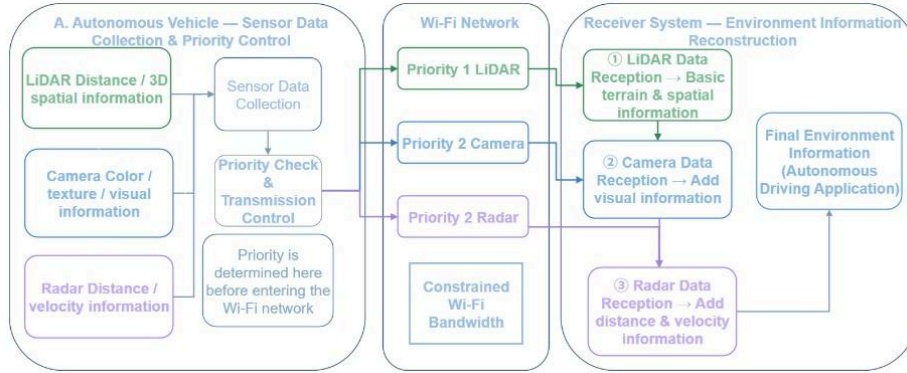
Figure 2. Priority Control and Transmission/Reception Flow of Wi-Fi-Based Multimodal Sensor Data for Indoor AMRs
