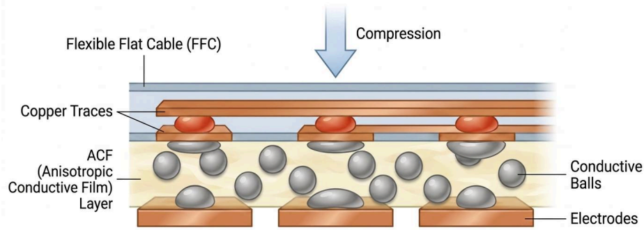
Figure 1. Conceptual cross-section of an ACF-bonded FFC joint. Compressed conductive particles form through-thickness current-transfer paths between opposing electrodes.
