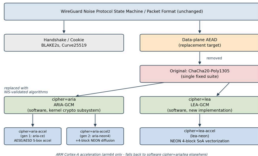
Figure 1. KWireGuard Architecture
