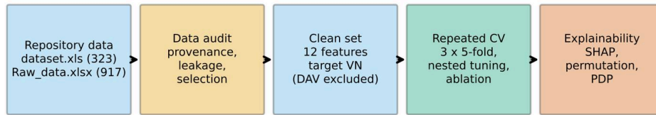
Figure 1. Study workflow.
